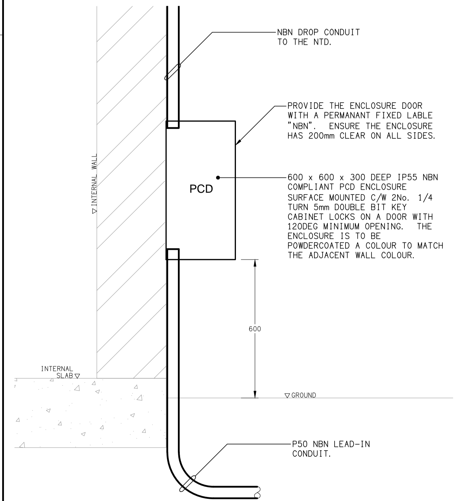
DETAIL PCD MOUNTING NOT TO SCALE
