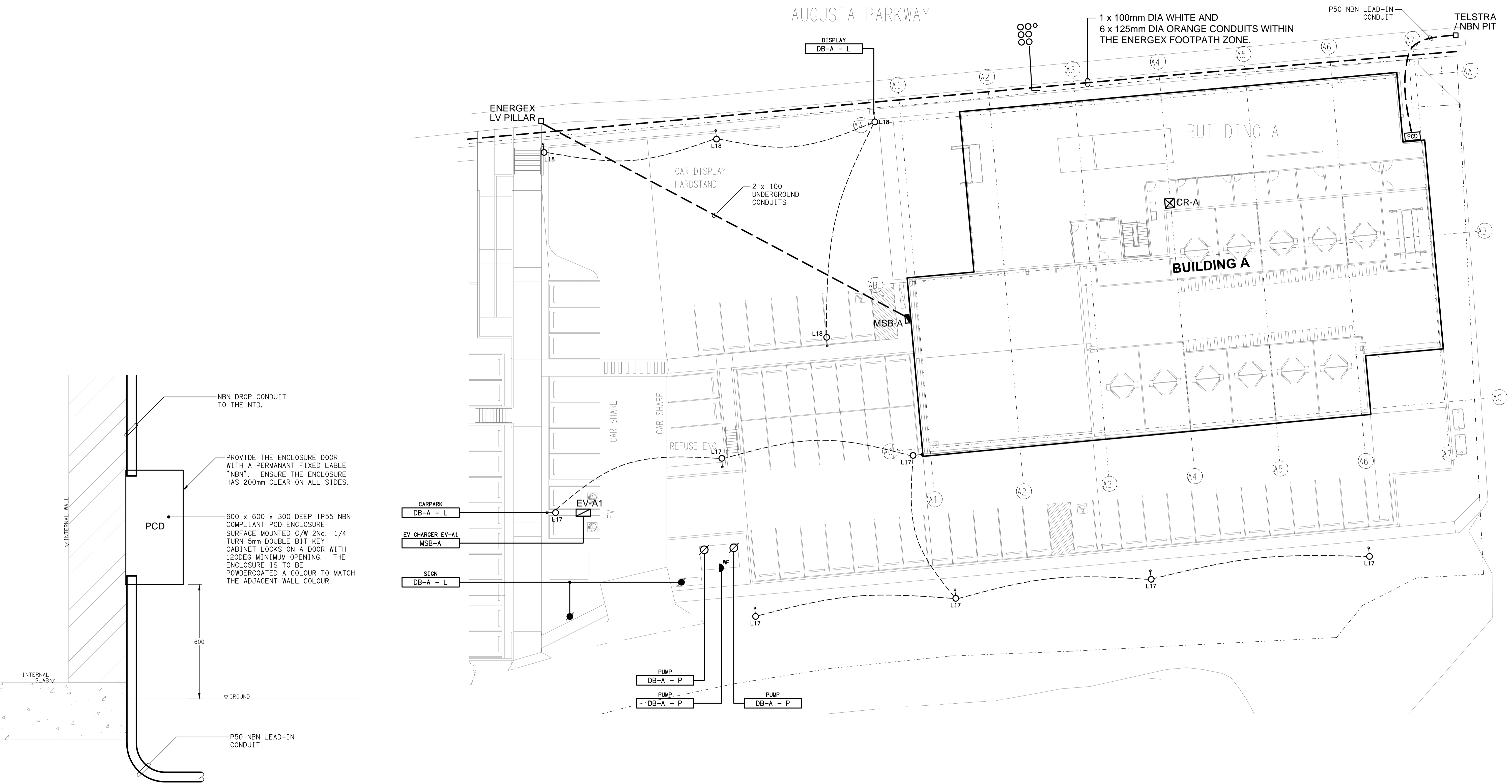
DETAIL PCD MOUNTING NOT TO SCALE
